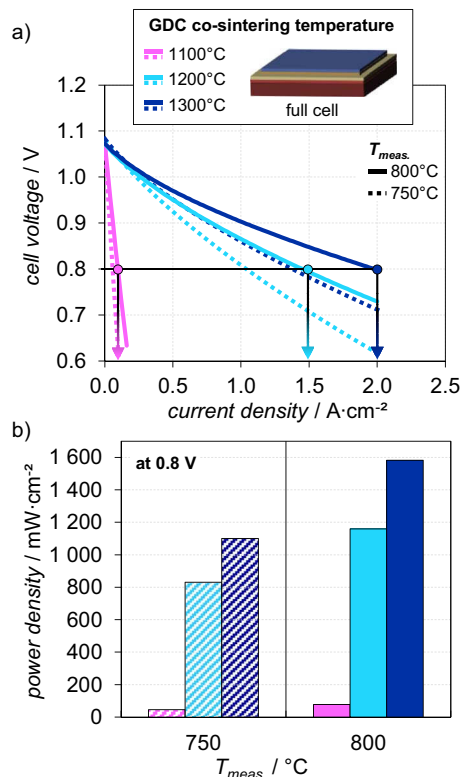
Figure 3. Performance evaluation of anode-supported cells with modified GDC co-sintering temperature, measured at T_{\text{meas.}} = 750 and 800^\circ\text{C} in syn. air ( p_{\text{O}_2} = 0.21\text{atm} ) at the cathode and 5.5% humidified \text{H}_2 at the anode; (a) current-voltage curves and corresponding (b) power density at 0.8 V.
